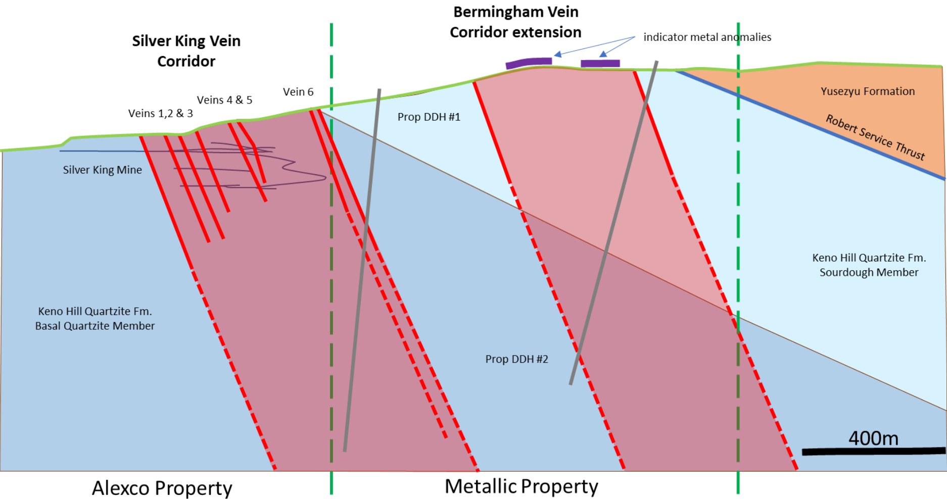
FIGURE 5 – SILVER QUEEN CROSS-SECTION
